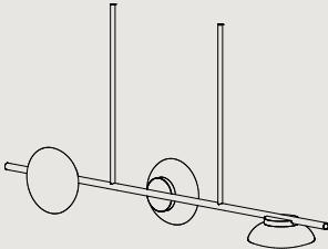
CHC23S* L 1306MM W 200MM H 200MM^ L 51.4" W 7.9" H 7.9"^^ CEILING CANOPY SPACING L 440MM / 17.32"
