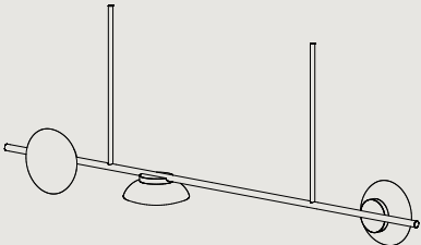
CHC24L* L 1706MM W 200MM H 200MM^ L 67.2" W 7.9" H 7.9"^^ CEILING CANOPY SPACING L 840MM / 33.07"
